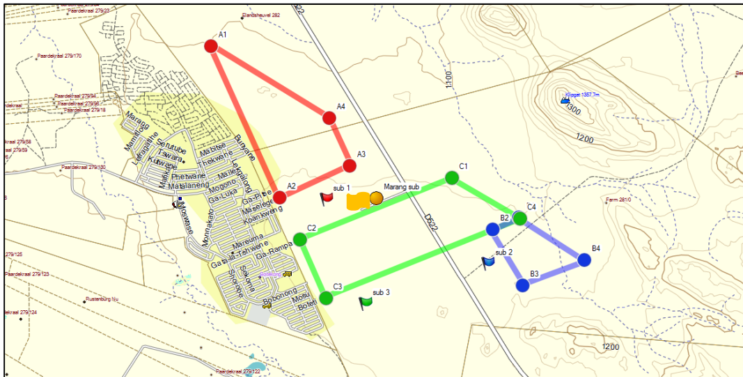
Figure 4: General corridor investigated for the new power lines between the new Marang Substation and the existing power lines. The red block = corridor 1 with the substation position indicated by the red flag, the blue block = corridor 2 with the substation position indicated by the blue flag, the green block = corridor 3 with the substation position indicated by the green flag and the extension to the existing substation (Alt 4) is marked with the yellow flag.
